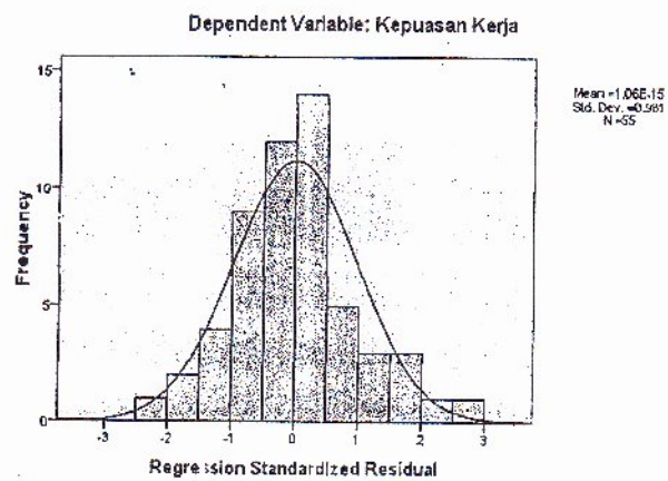
Histogram
