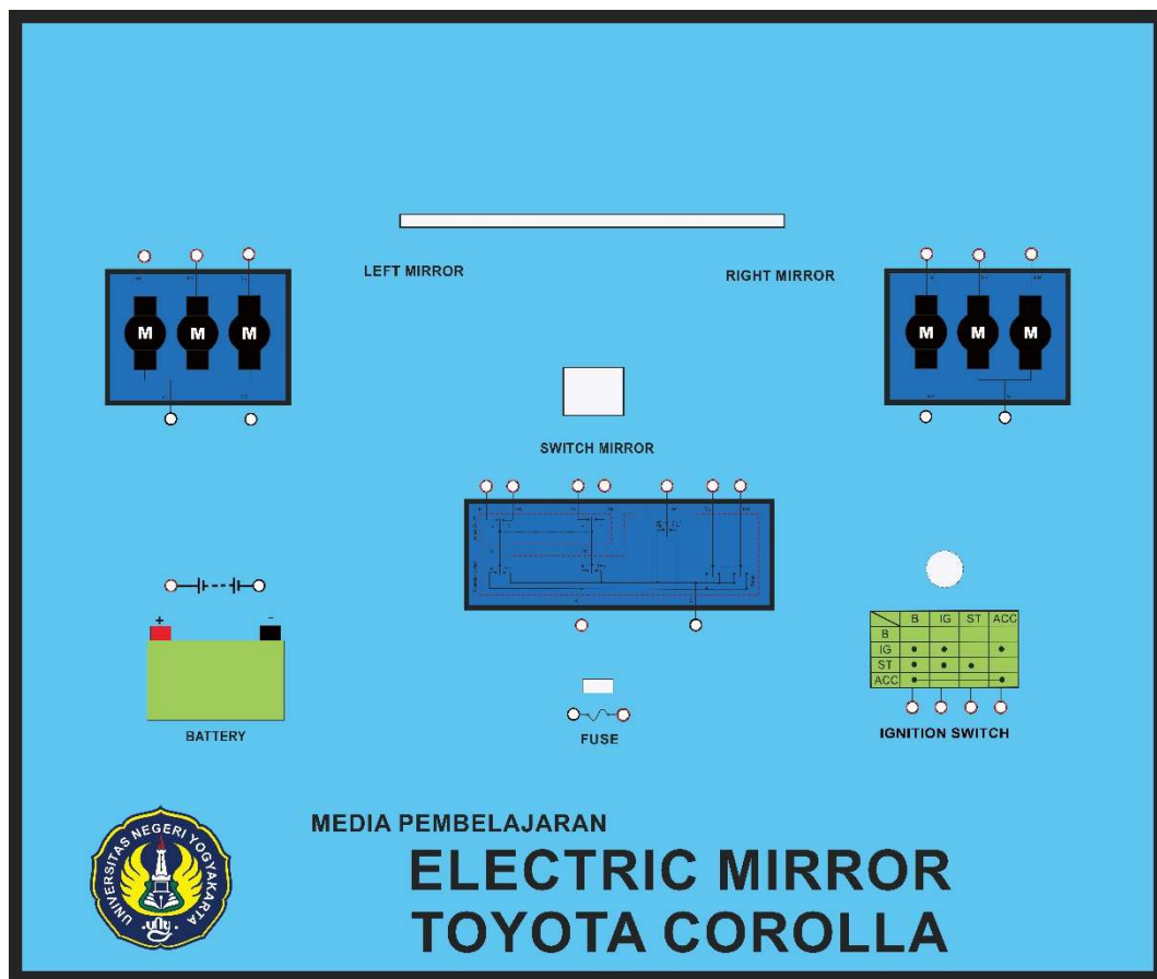
Lampiran 4. Desain Layout simulator Electric Mirror
