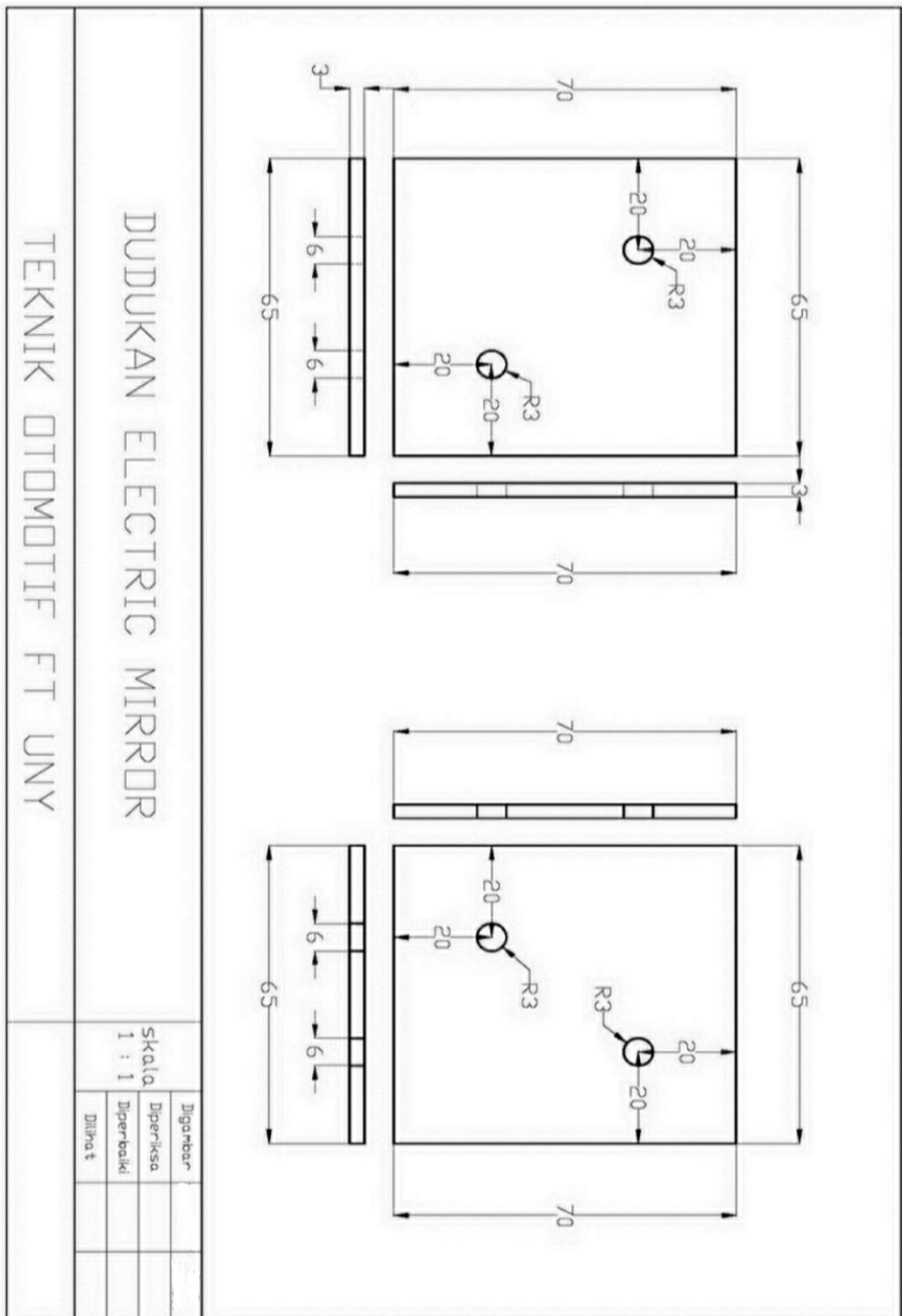
Lampiran 2. Dudukan Electric Mirror
