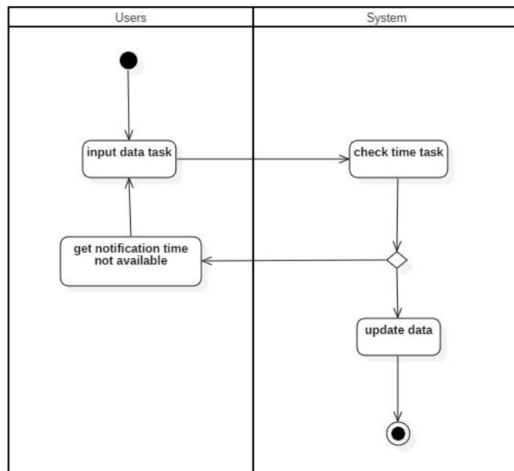
Gambar 26. Activity Diagram Edit Task
