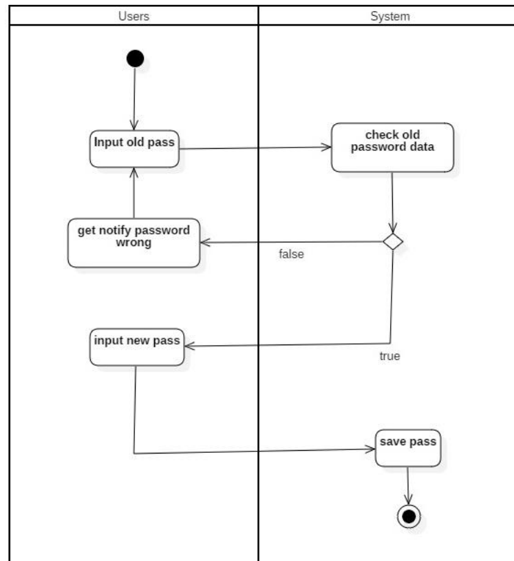
Gambar 20. Activity Diagram Edit Password
