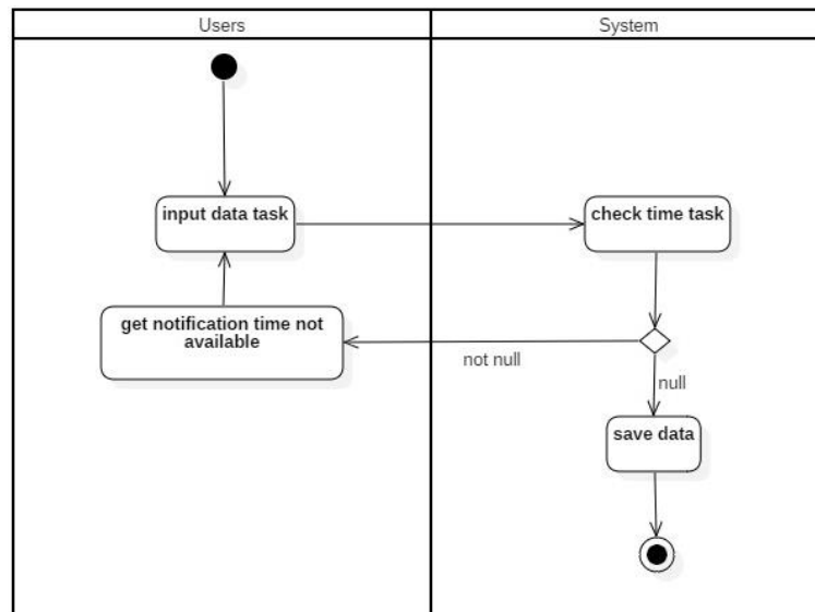
Gambar 24. Activity Diagram Add Task
