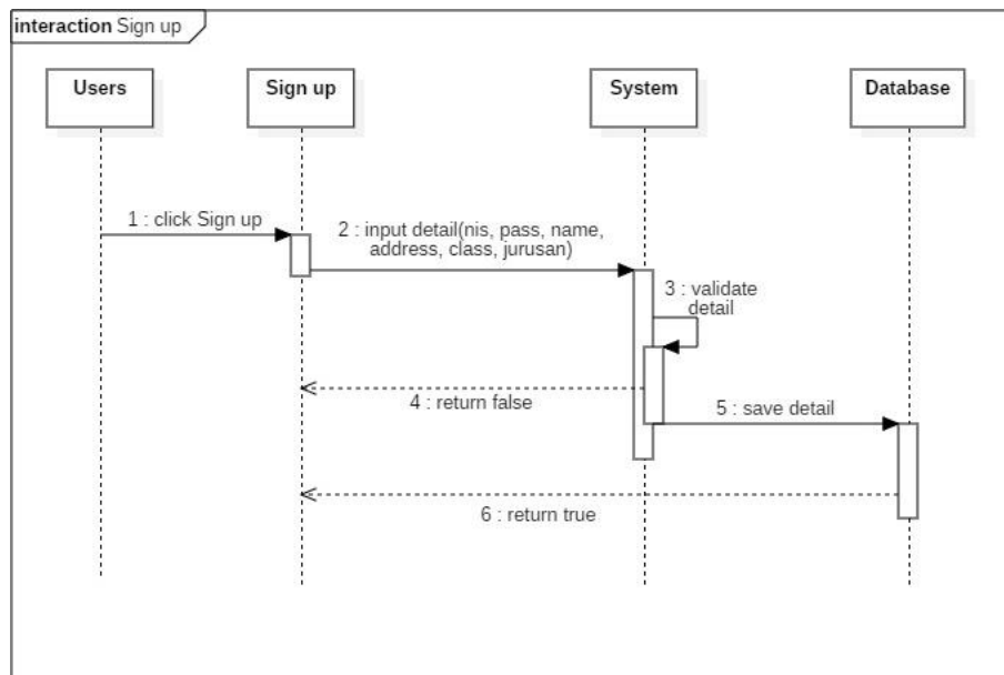
Gambar 2. Sequence Diagram Sign in
