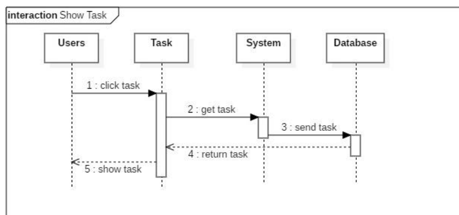
Gambar 7. Sequence Diagram Show Task
