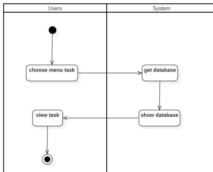
Gambar 23. Activity Diagram Task
