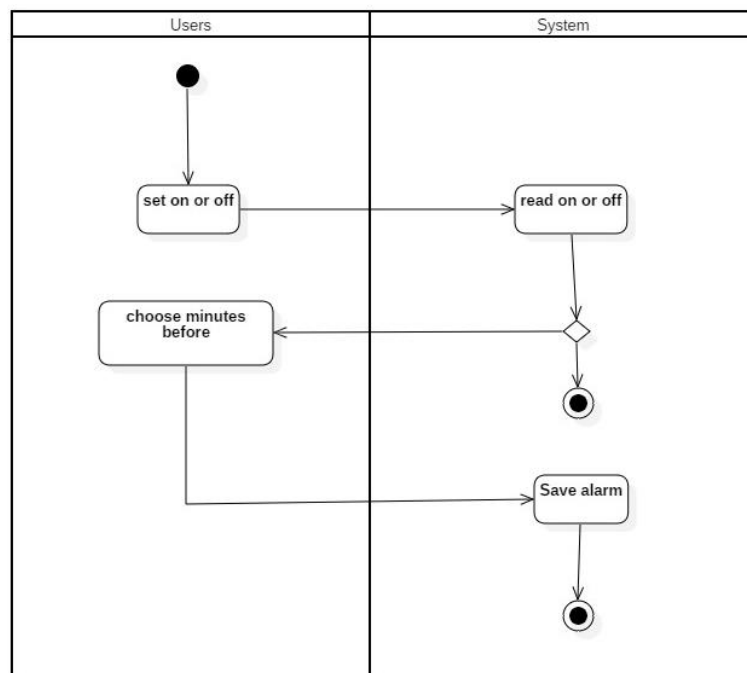
Gambar 29. Activity Diagram Set Alarm Minutes Before
