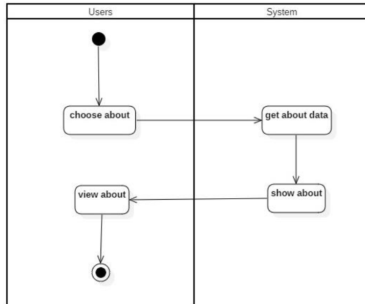
Gambar 30. Activity Diagram Set Alarm Day Before
