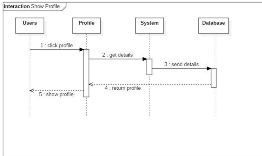
Gambar 3. Sequence Diagram Show profile
