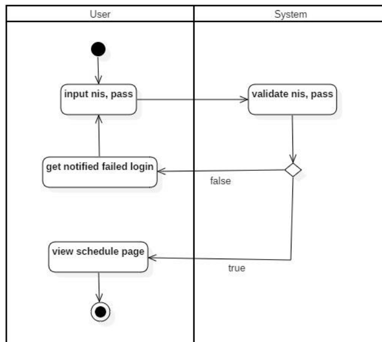
Gambar 17. Activity Diagram Sign in
