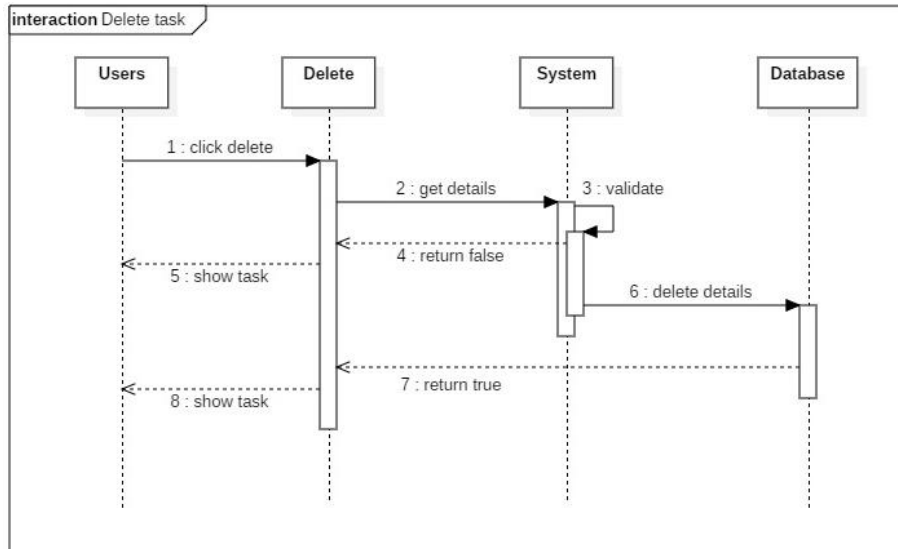
Gambar 10. Sequence Diagram Delete Task
