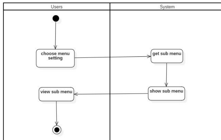
Gambar 27. Activity Diagram Setting Notification
