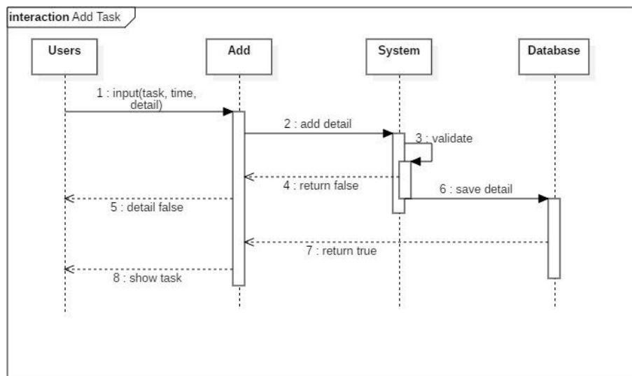
Gambar 11. Sequence Diagram Add task
