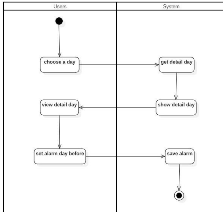
Gambar 28. Activity Diagram Set Alarm Day Before
