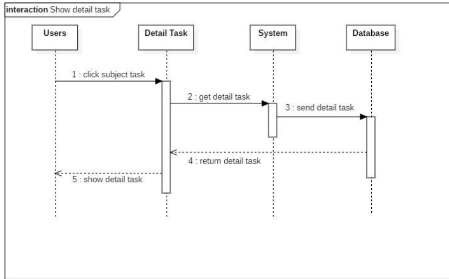
Gambar 8. Sequence Diagram Show detail task
