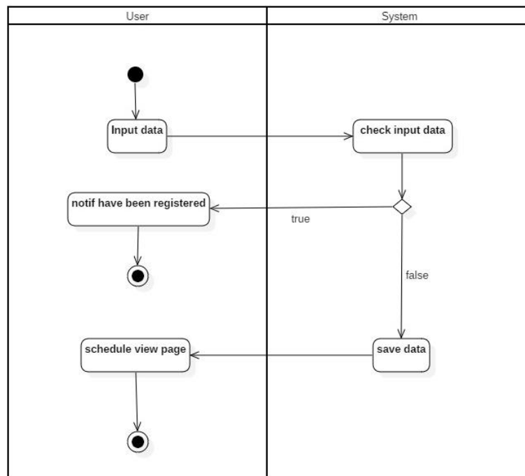
Gambar 18. Activity Diagram Sign up
