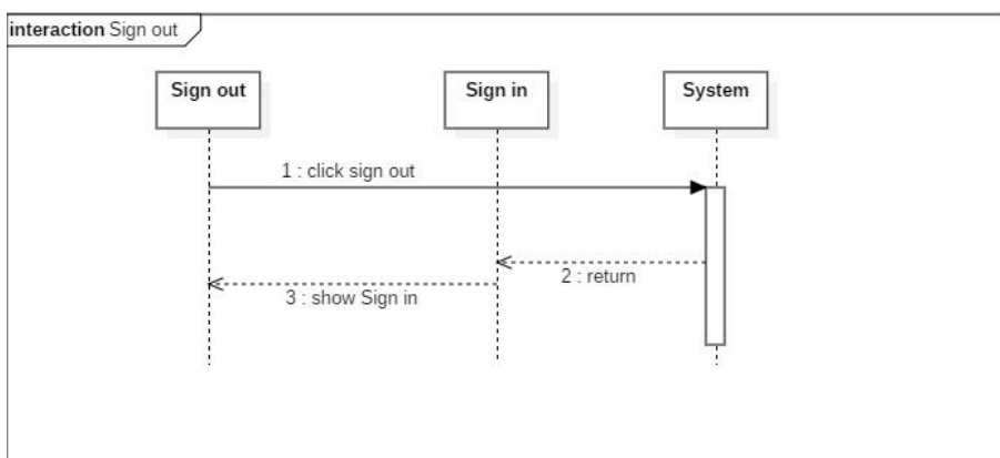
Gambar 16. Sequence Diagram Sign out
