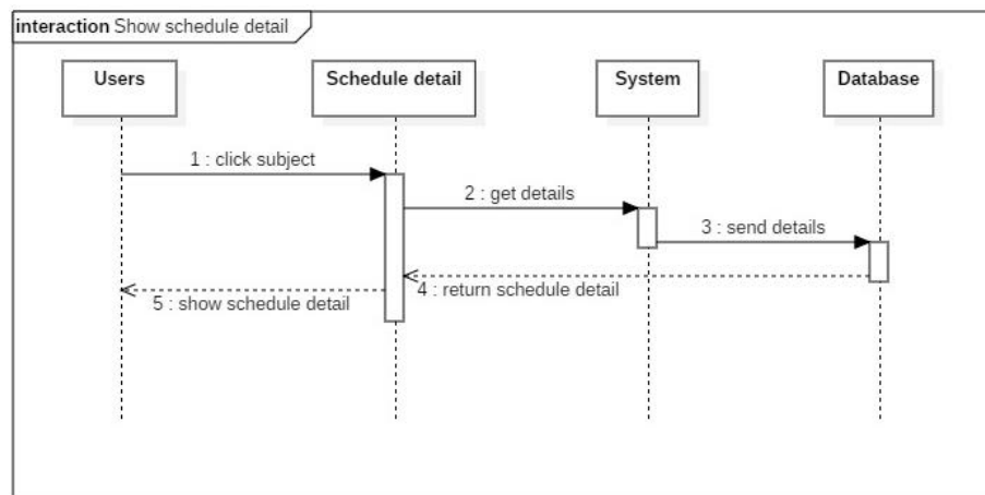
Gambar 6. Sequence Diagram Show Schedule Detail
