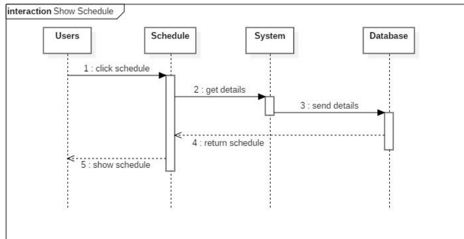
Gambar 5. Sequence Diagram Show Schedule
