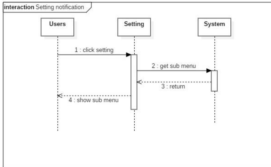
Gambar 12. Sequence Diagram Setting notification
