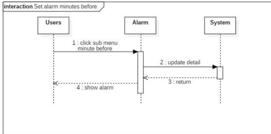
Gambar 14. Sequence Diagram Set Alarm Minutes before
