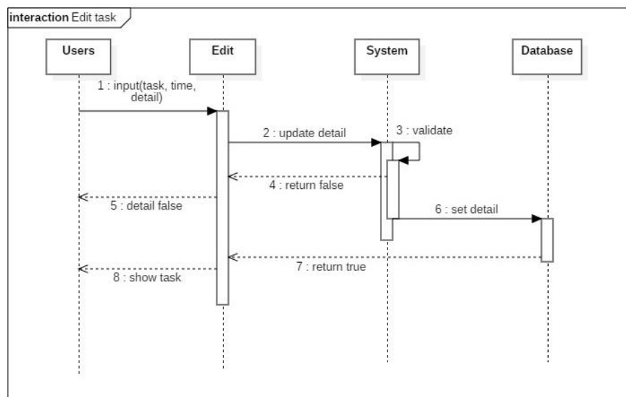
Gambar 9. Sequence Diagram Edit Task
