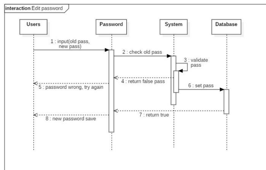
Gambar 4. Sequence Diagram Edit Password
