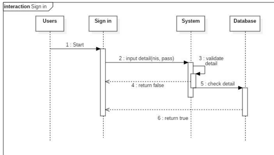
Gambar 1. Sequence Diagram Sign in
