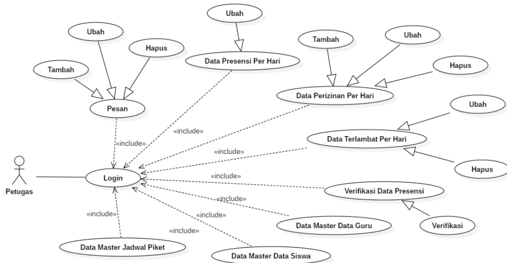
Gambar 2. Use Case Diagram Petugas
