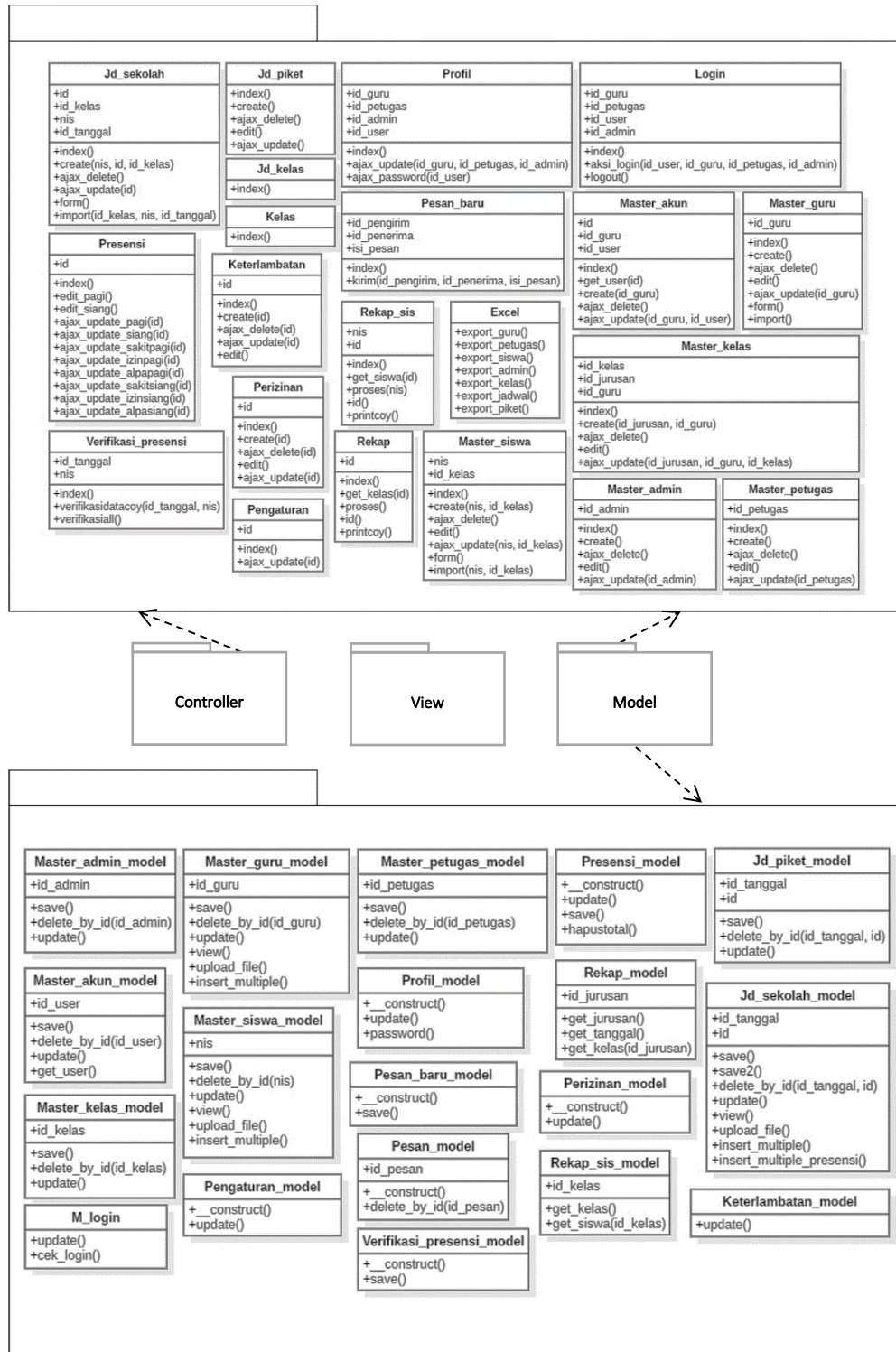
Gambar 4. Class Diagram
