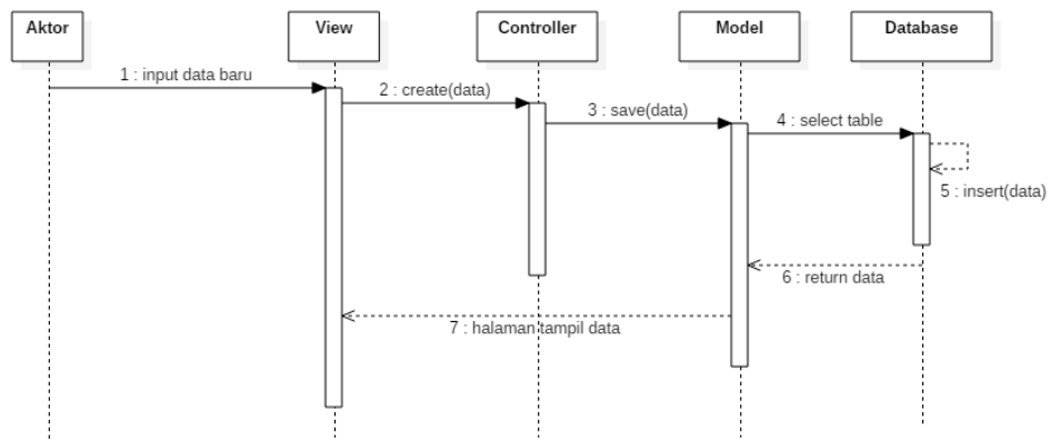
Gambar 6. Sequence Diagram Tambah Data
