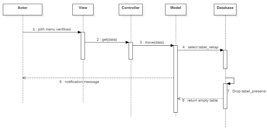
Gambar 12. Sequence Diagram Presensi Siswa
