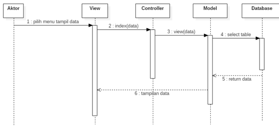
Gambar 11. Sequence Diagram Lihat Data
