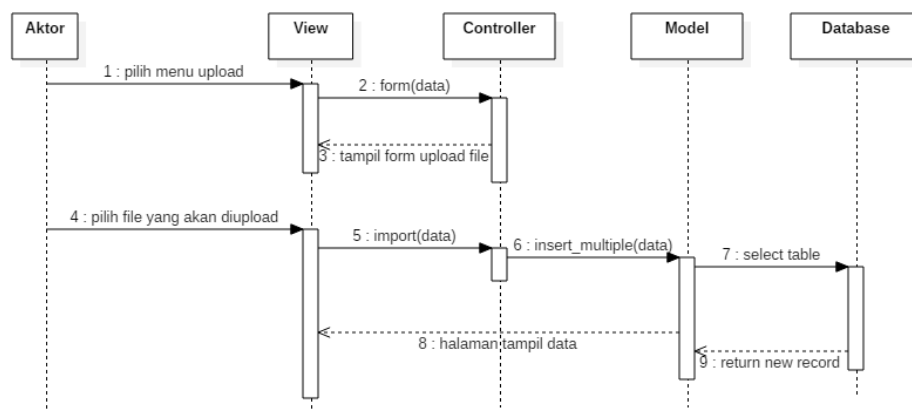
Gambar 9. Sequence Diagram Import Data
