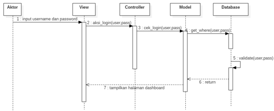
Gambar 5. Sequence Diagram Login
