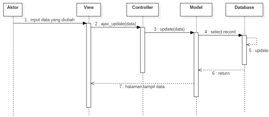
Gambar 8. Sequence Diagram Ubah Data
