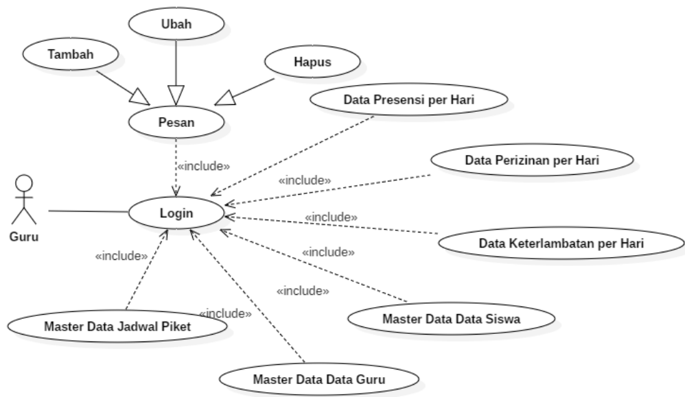
Gambar 3. Use Case Diagram Guru
