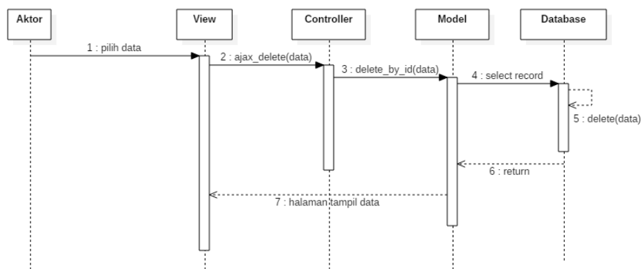
Gambar 7. Sequence Diagram Hapus Data
