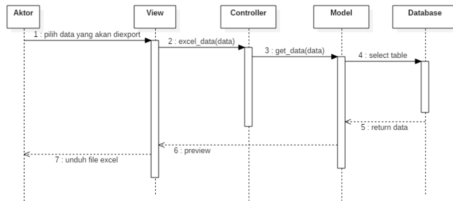
Gambar 10. Sequence Diagram Export Data
