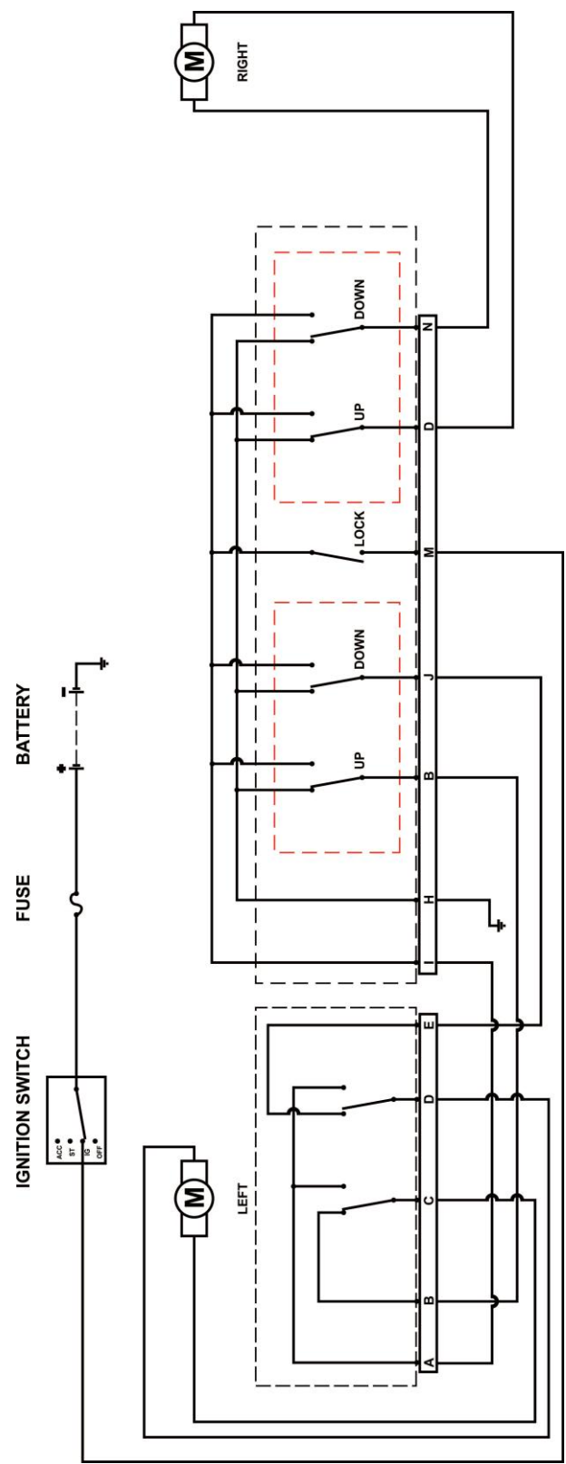
Lampiran 5. Gambar Rangkaian Sistem Power Window Timor
