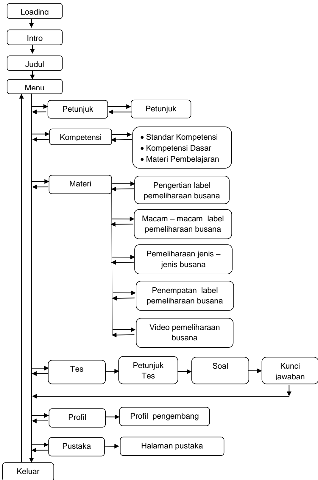
Gambar 9. Flowchart View
