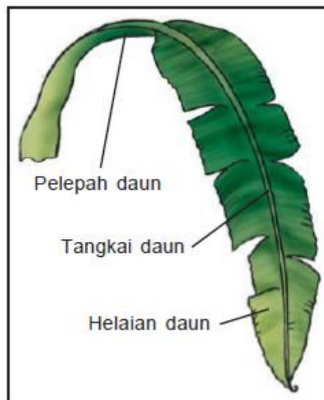
Gambar 2.6 Bagian-bagian daun.
