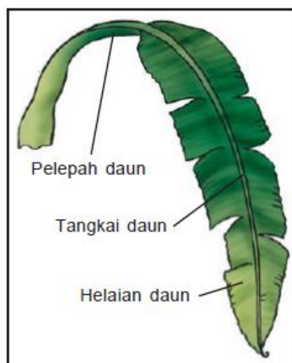
Bagian-bagian daun
