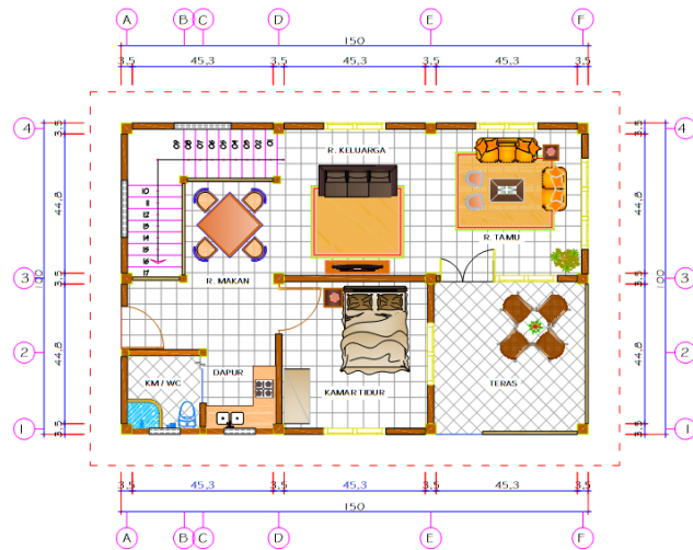
Gambar 5. Denah Lantai 1
