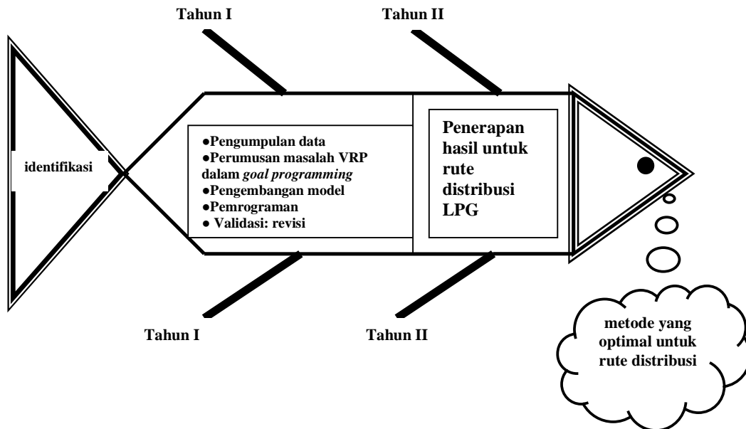
Gambar 1. Diagram Fishbone
