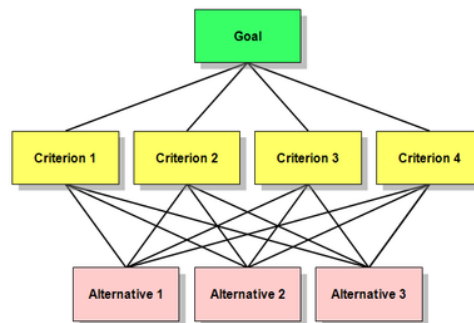
Gambar 4. Struktur Hirarki AHP (Forman & Gass, 2001)
