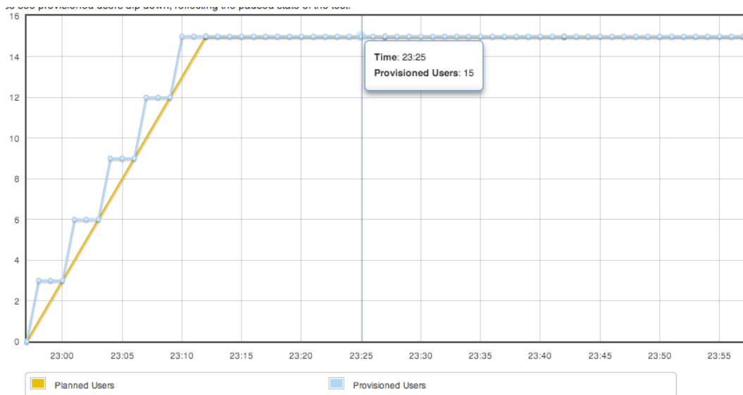
Gambar 26. Hasil pengujian reliability
