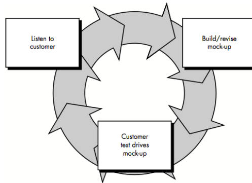
Gambar 6. Paradigma Model Pengembangan Prototype (Pressman, 2010)
