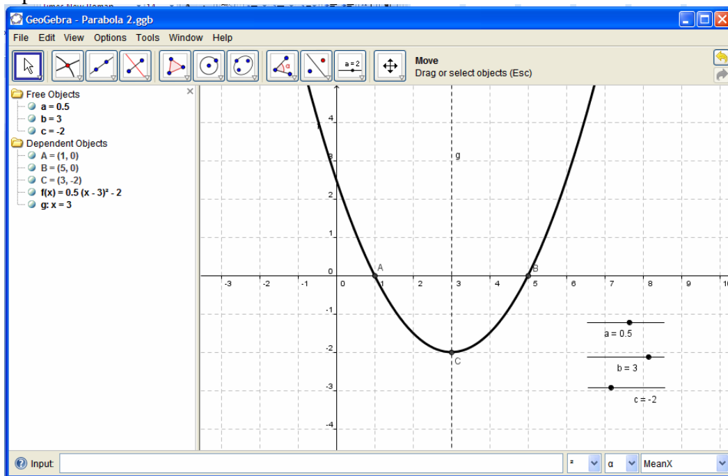
Gambar 7. Parabola
